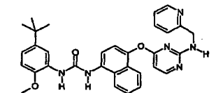
1-(5-tert-Butyl-2-methoxy-phenyl)-3-(4-{2-[(pyridin-2-ylmethyl)-amino]-pyrimidin-4-yloxy}-naphthalen-1-yl)-urea;
